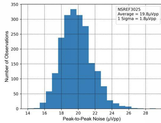
Figure 7-20 0.1Hz to 10Hz Noise Histogram
