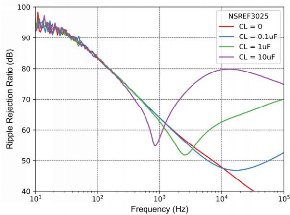
Figure 7-9 Ripple Rejection Ratio vs. Frequency
