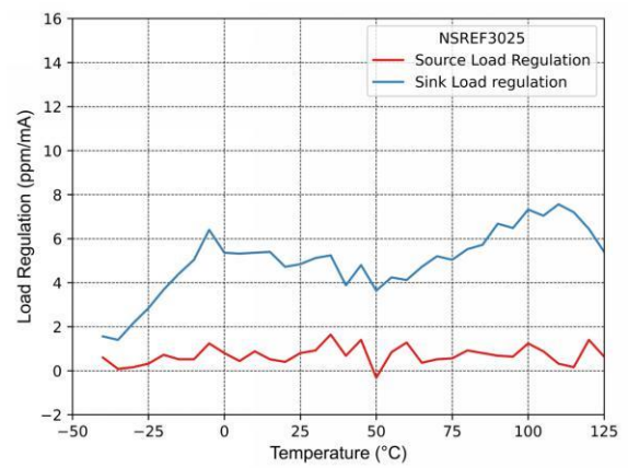
Figure 7-8 Load Regulation vs Temperature (-40°C to 125°C)
