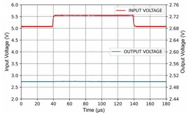
Figure 7-12 Line Transient Response (CL=1uF)
