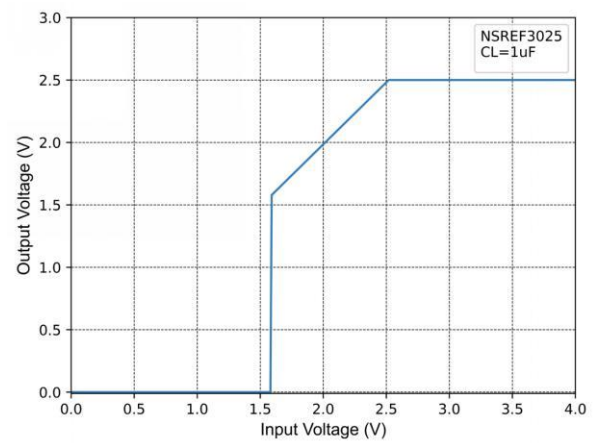
Figure 7-4 Output Voltage vs. Input Voltage
