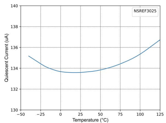
Figure 7-6 Quiescent Current vs Temperature (-40°C to 125°C)
