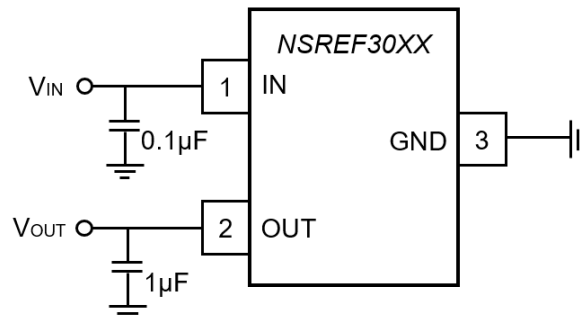
Figure 8.1 Typical Connections for Operating NSREF30xx
