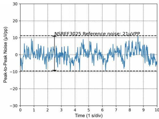
Figure 7-19 0.1Hz to 10Hz Voltage Noise
