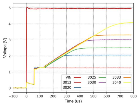
Figure 7-18 Step Response
