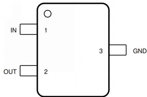
Figure 1.1 NSREF30xx Package
