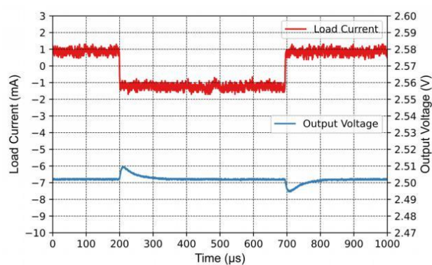
Figure 7-14 Load Transient Response \pm 1\text{mA} ( \text{CL}=1\mu\text{F} )
