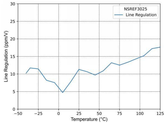
Figure 7-7 Line Regulation vs Temperature (-40°C to 125°C)
