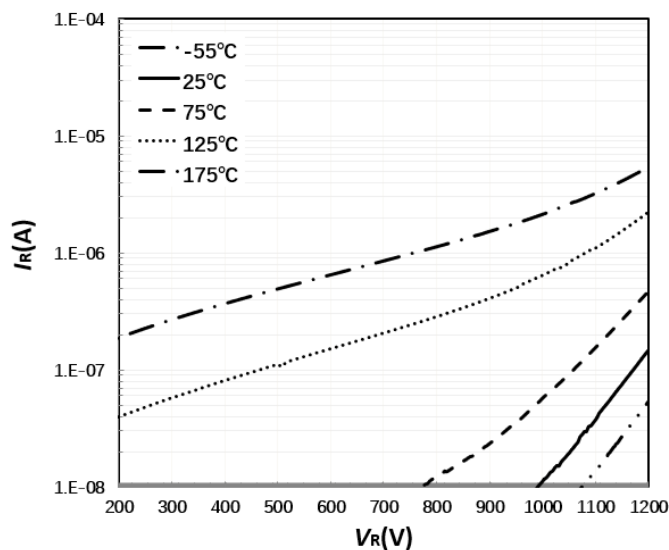
Figure 2. Typical reverse characteristic
