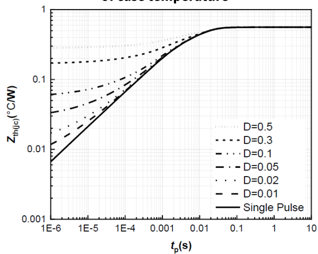
Figure 7. Max transient thermal impedance
