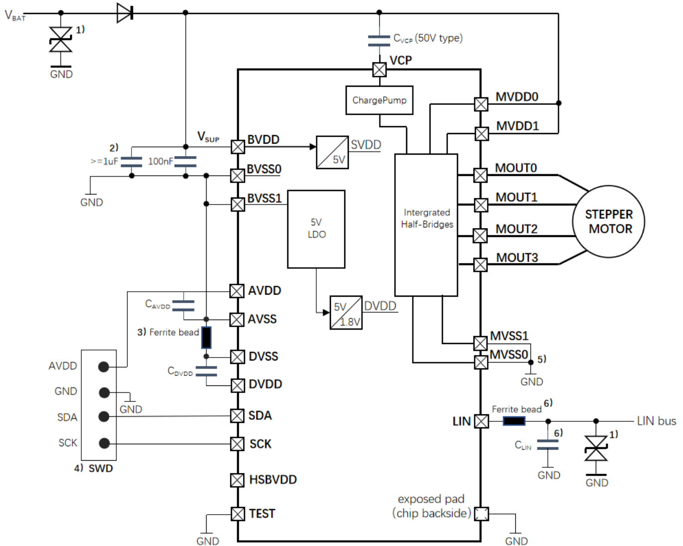
Figure 6.1 Typical application diagram
