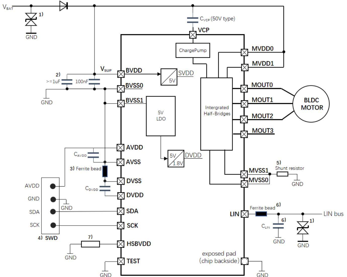
Figure 6.2 Typical application diagram
