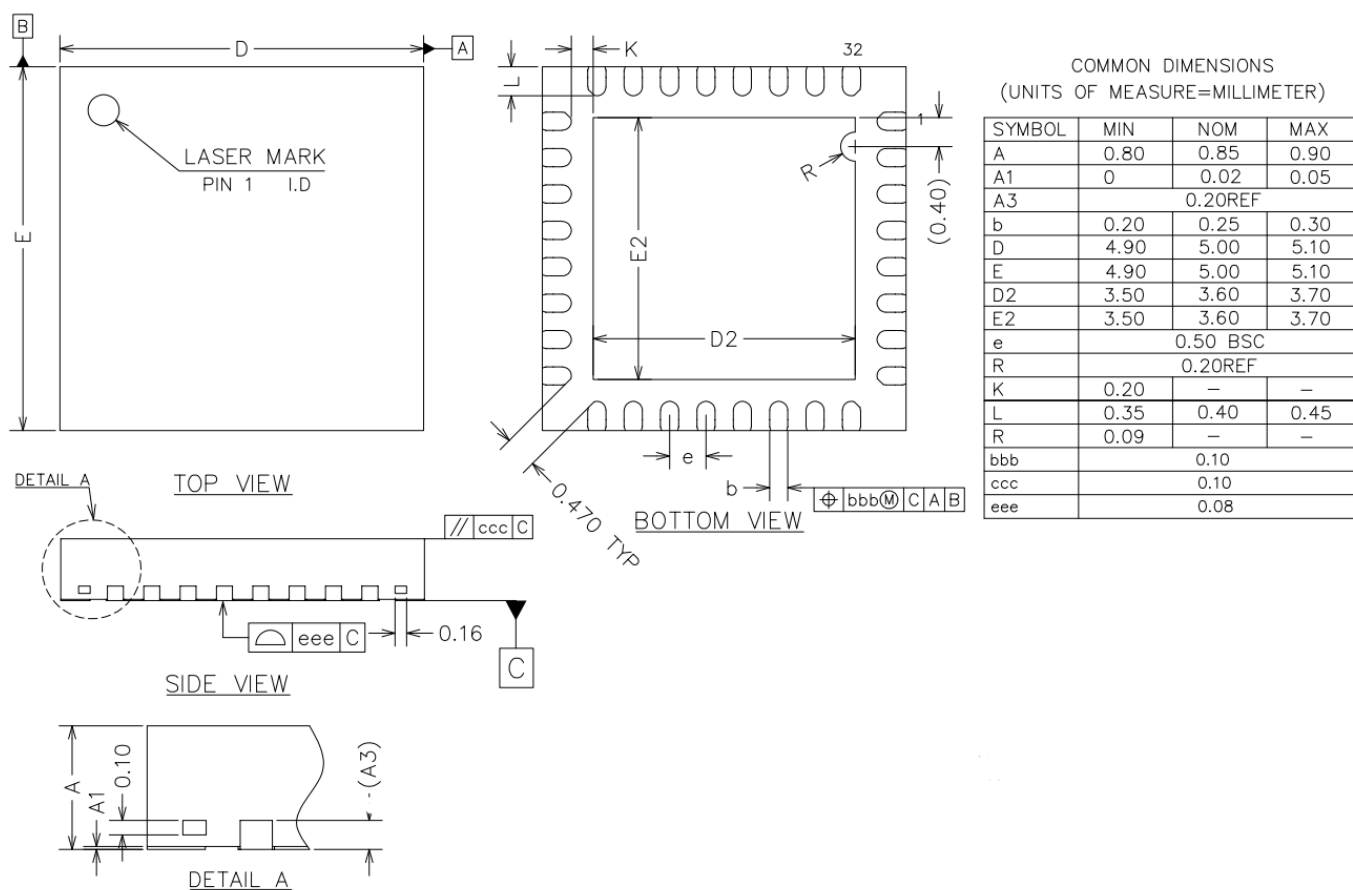
Figure 7.1 QFN32(5*5) Package Shape and Dimension in millimeters and (inches)
